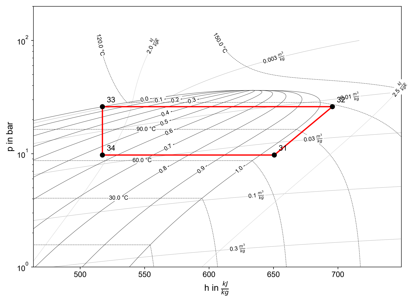
Cycle 2 (R600a)
