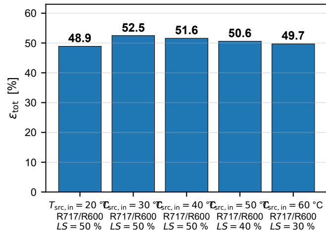
Exergetic efficiency
