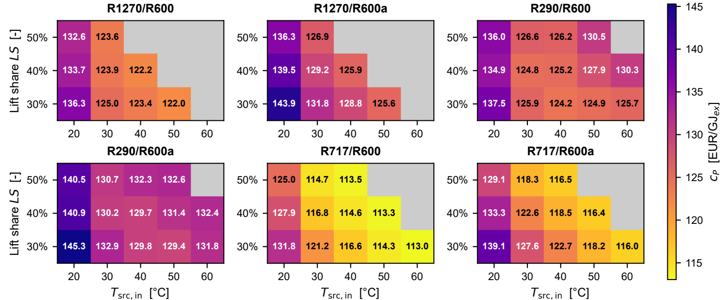
C_p heatmap per design ( T_{\text{steam}} = 110\text{ }^{\circ}\text{C} )
