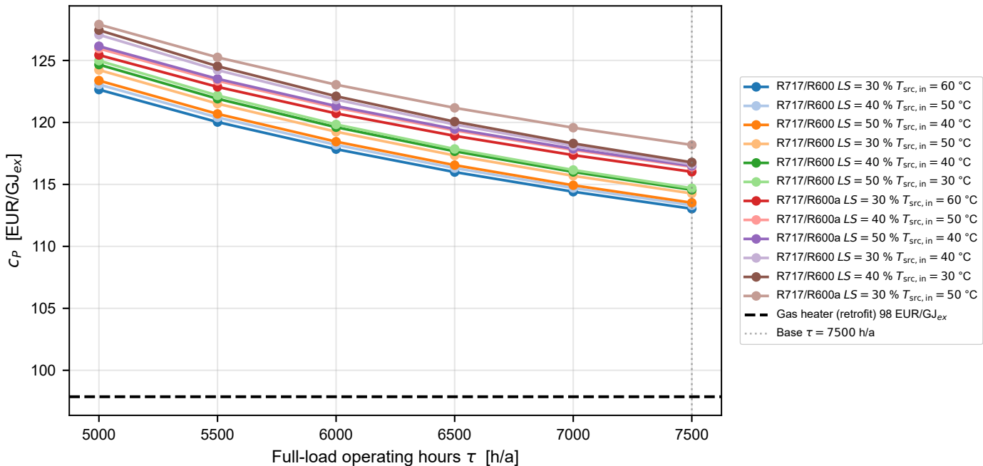
C_P vs full-load hours — 12 cheapest designs ( T_{\text{steam}} = 110\text{ °C} )
