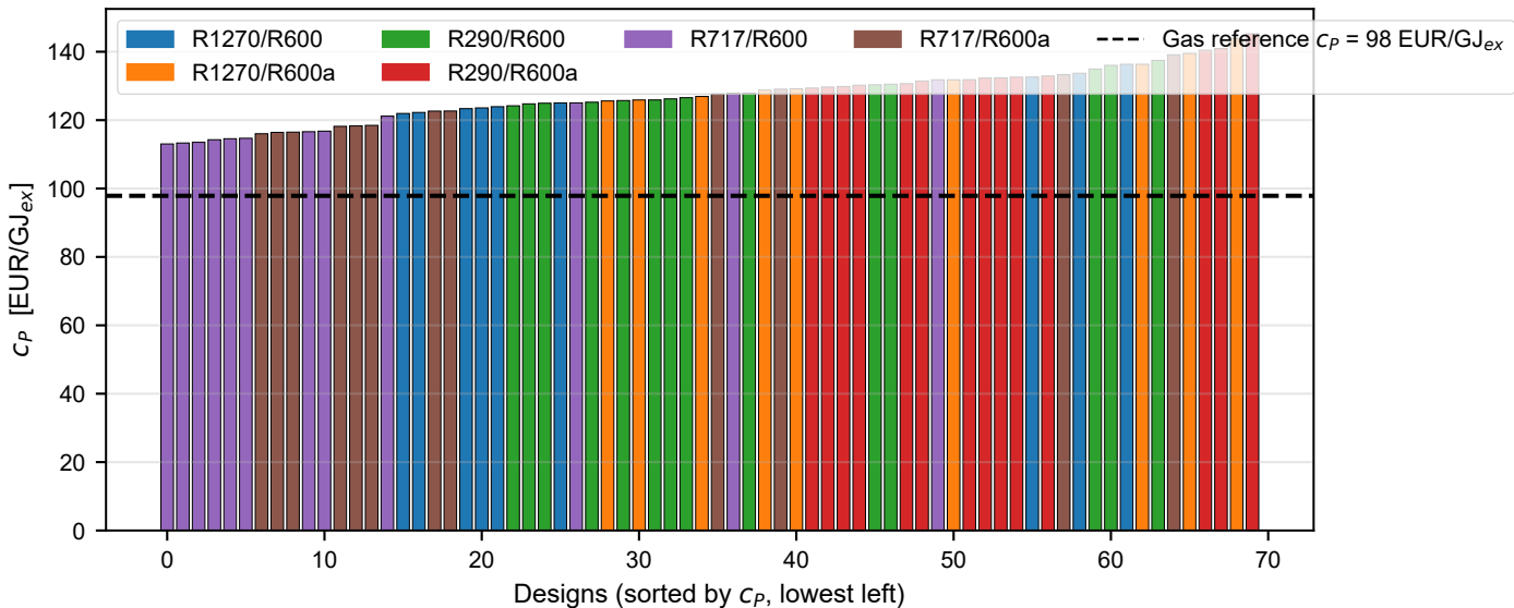
c_p — all OK designs sorted ( T_{\text{steam}} = 110\text{ °C} )
