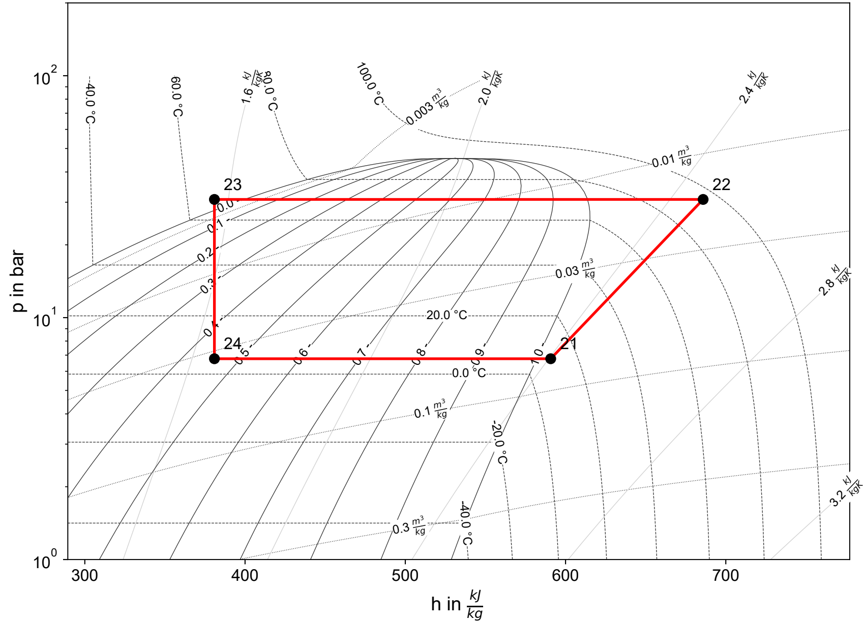
Cycle 1 (R1270)
