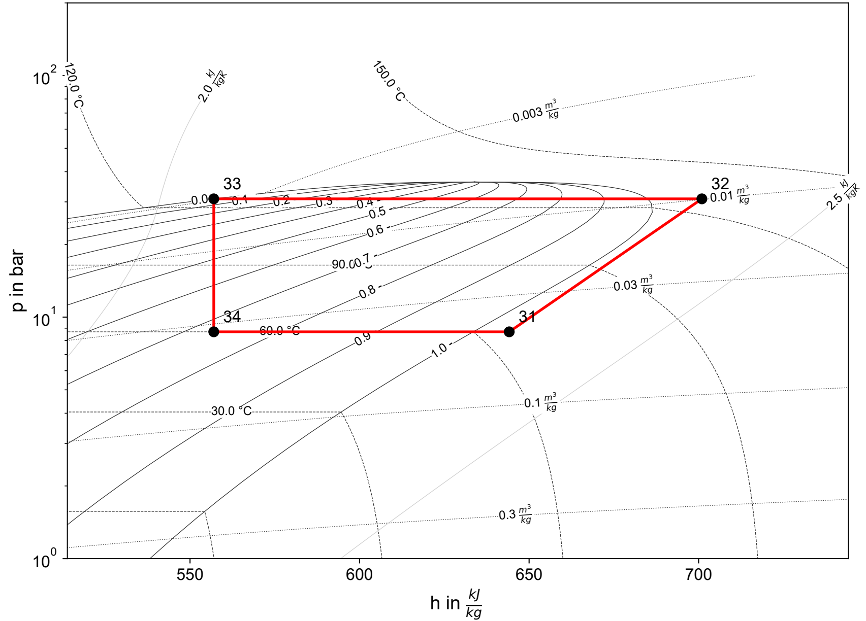
Cycle 2 (R600a)
