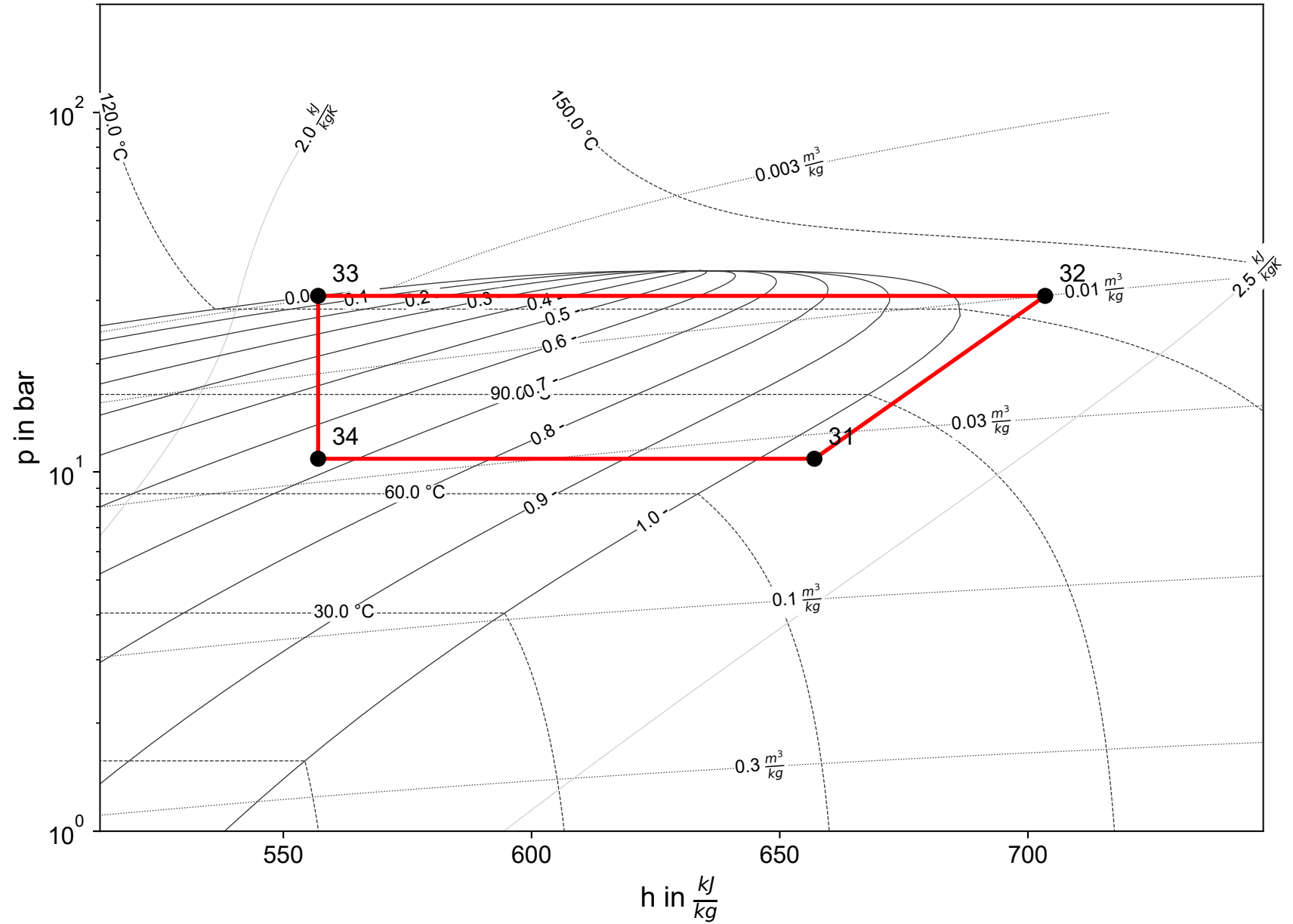
Cycle 2 (R600a)
