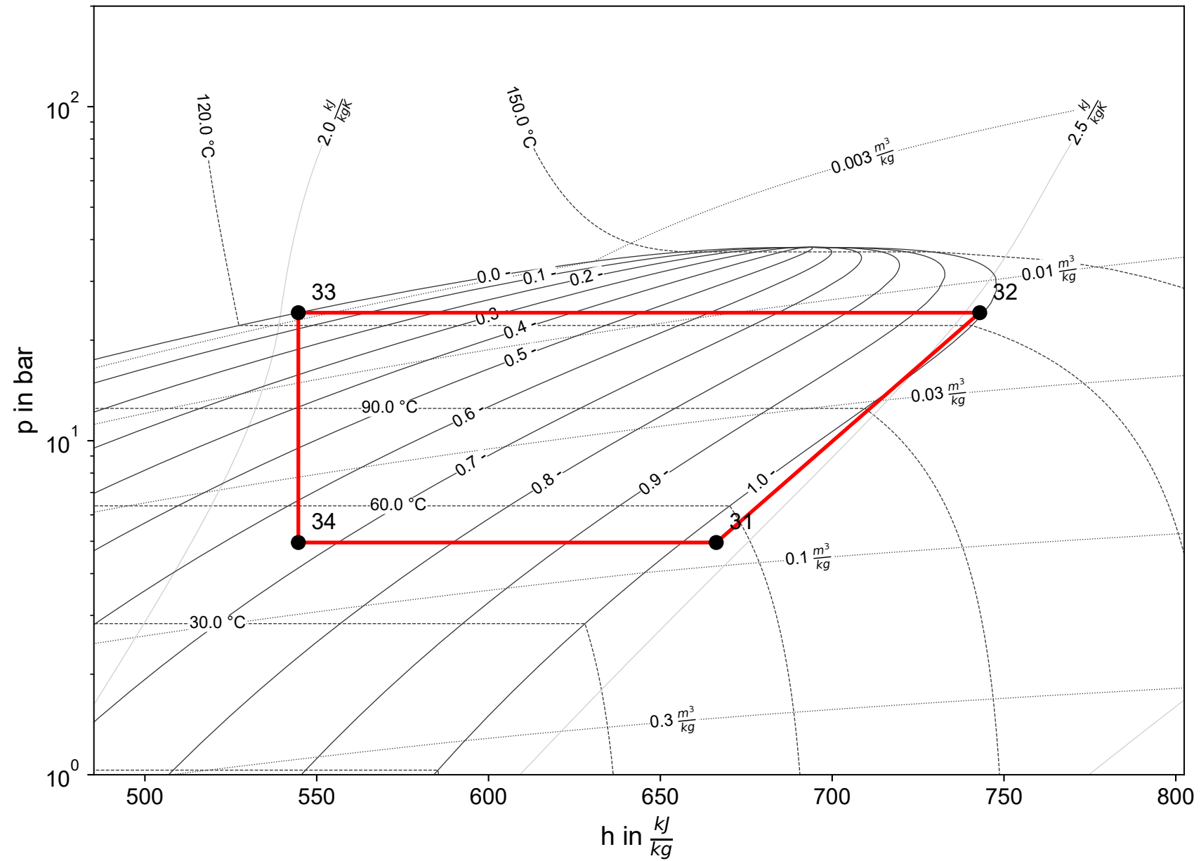
Cycle 2 (R600)
