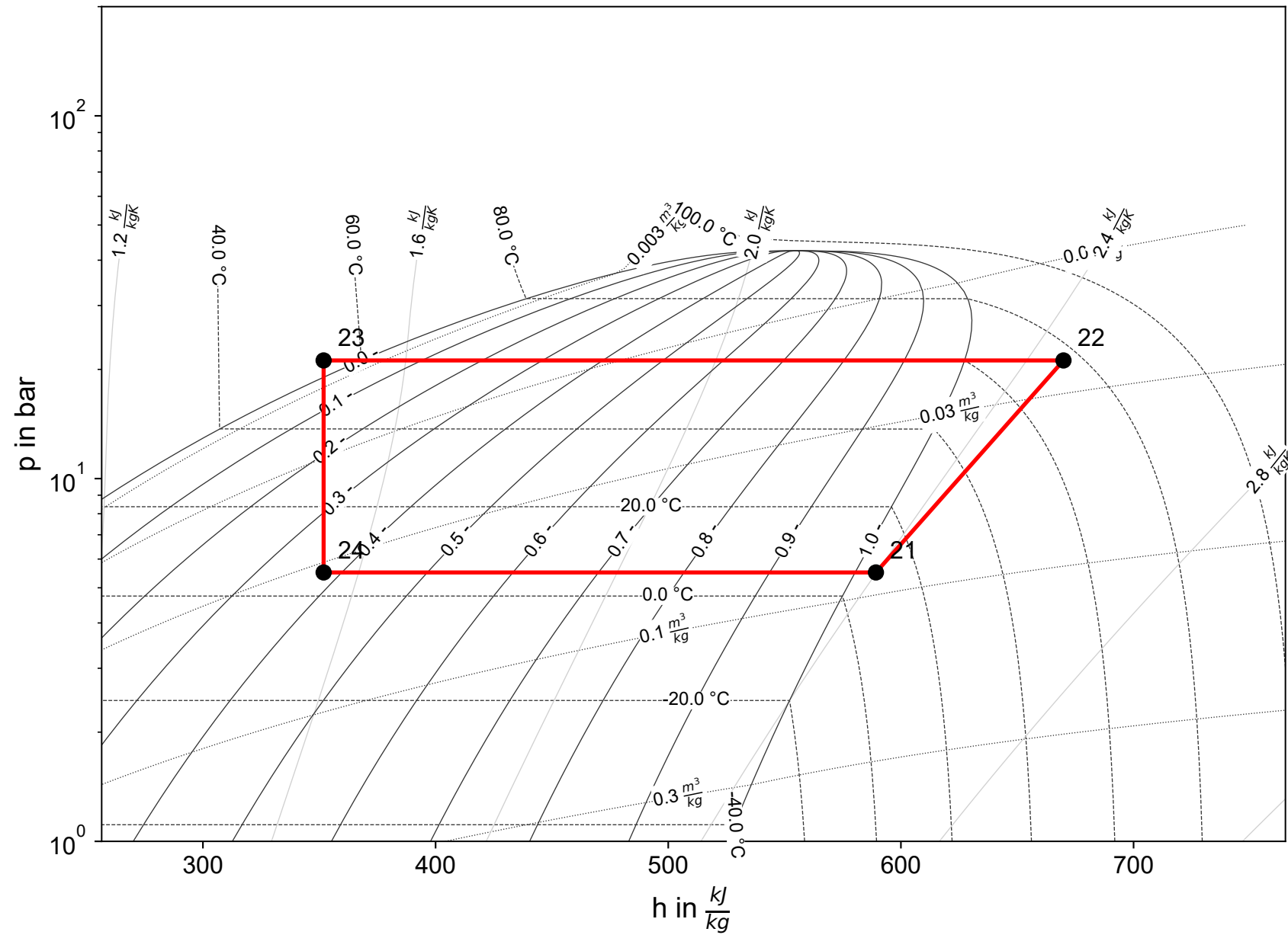
Cycle 1 (R290)
