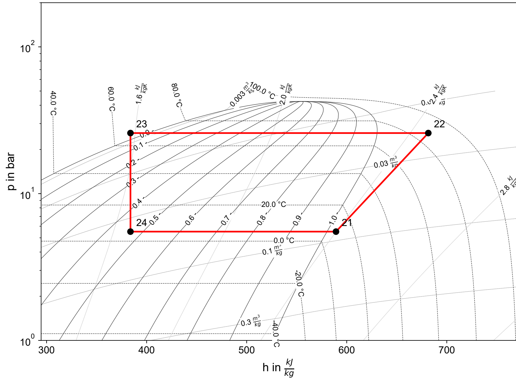
Cycle 1 (R290)
