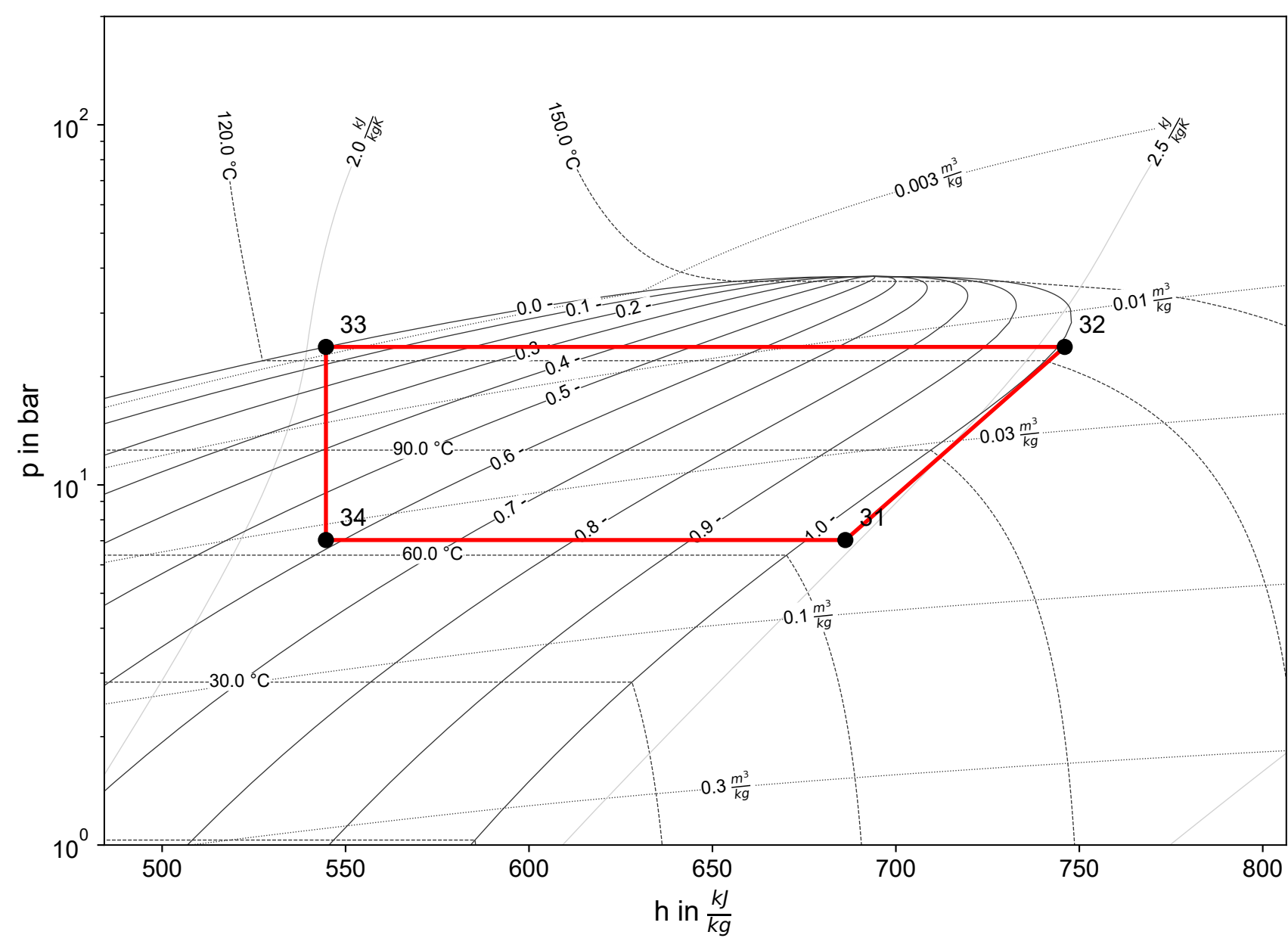
Cycle 2 (R600)
