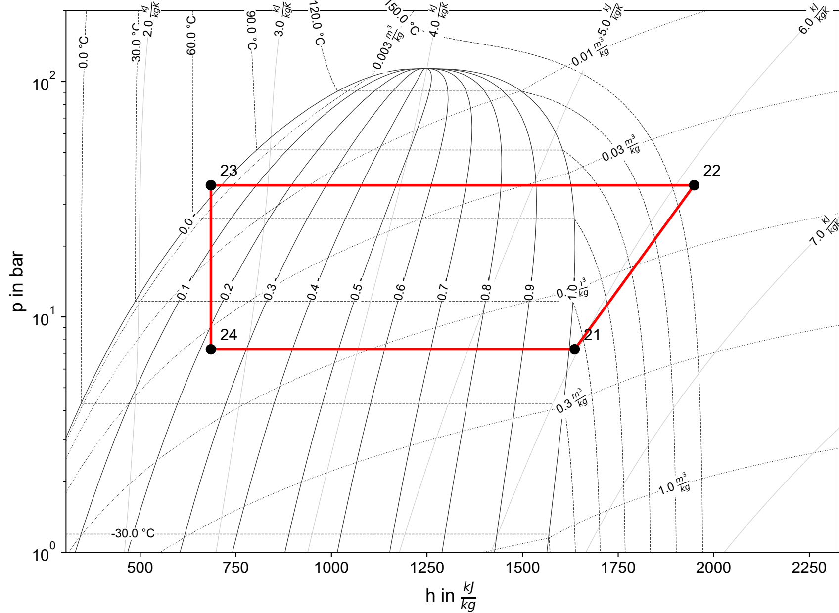
Cycle 1 (R717)
