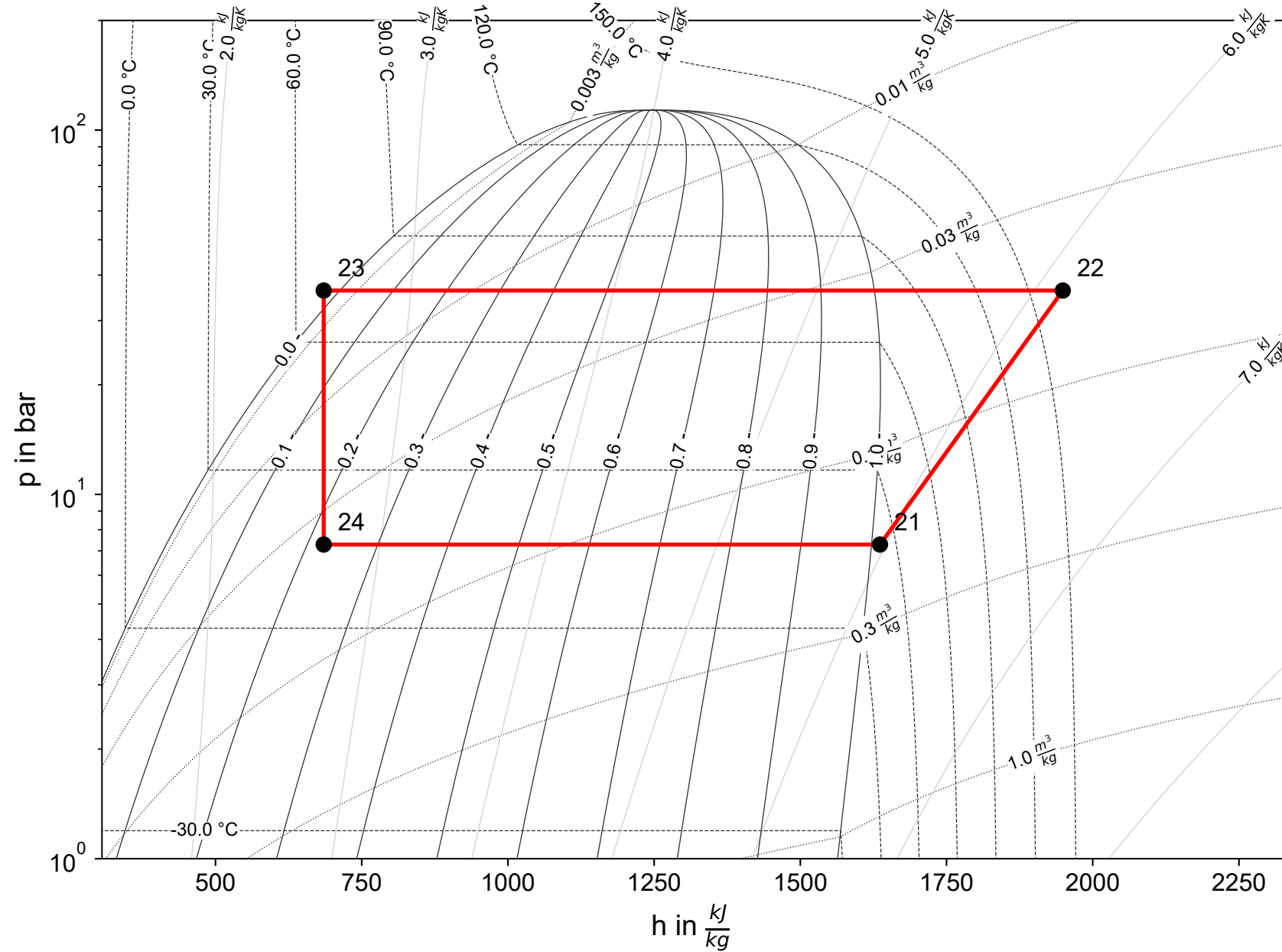
Cycle 1 (R717)
