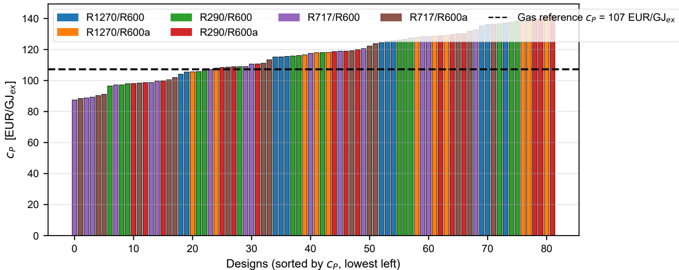
c_p — all OK designs sorted ( T_{\text{steam}} = 100\text{ }^{\circ}\text{C} )
