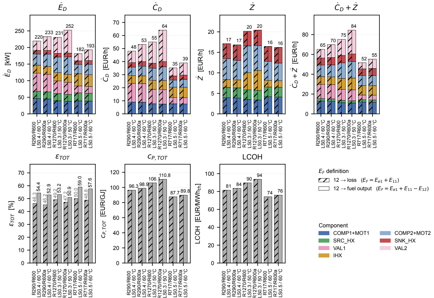
E_F definition comparison — cost-optimal design per pair, T_{\text{steam}} = 110\text{ }^{\circ}\text{C} (only \varepsilon_{TOT} responds; all destruction and cost metrics are invariant)
