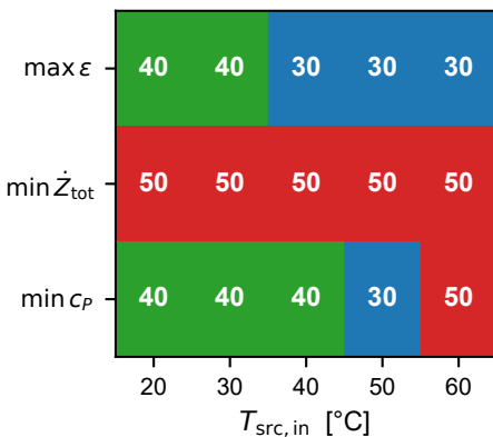
R290/R600a
