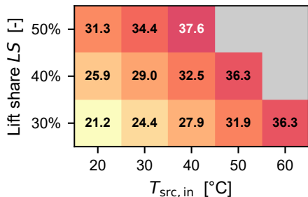
R290/R600a
