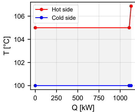
Sink HX (cycle-2 condenser, steam)
