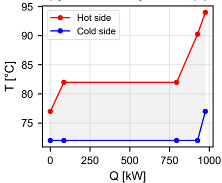
Internal HX (cycle-1 cond. / cycle-2 evap.)
