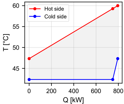
Source HX (cycle-1 evaporator)
