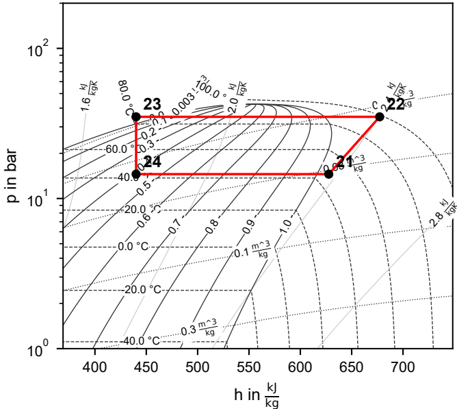
Cycle 1 (R290)
