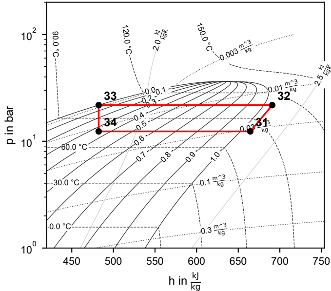
Cycle 2 (R600a)
