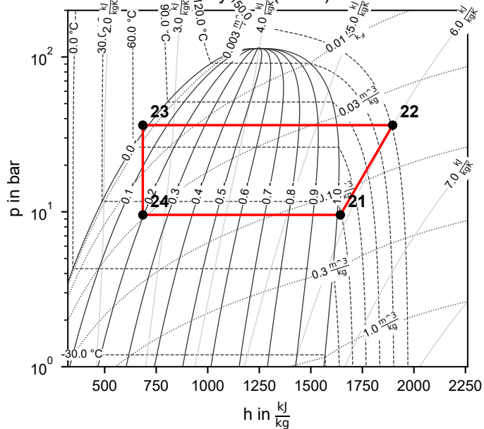
Cycle 1 (R717)
