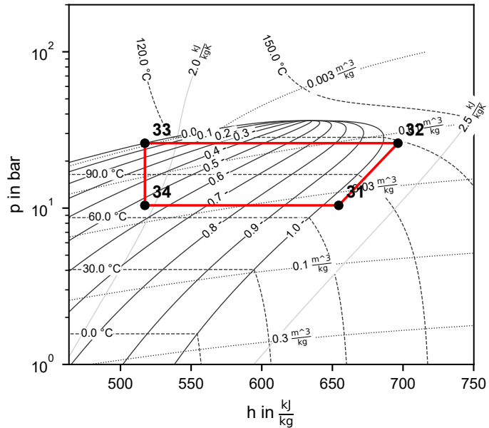
Cycle 2 (R600a)
