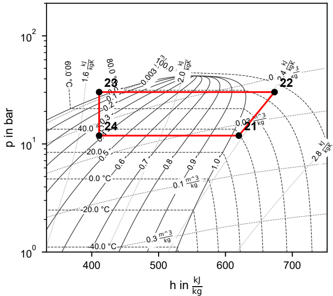
Cycle 1 (R290)
