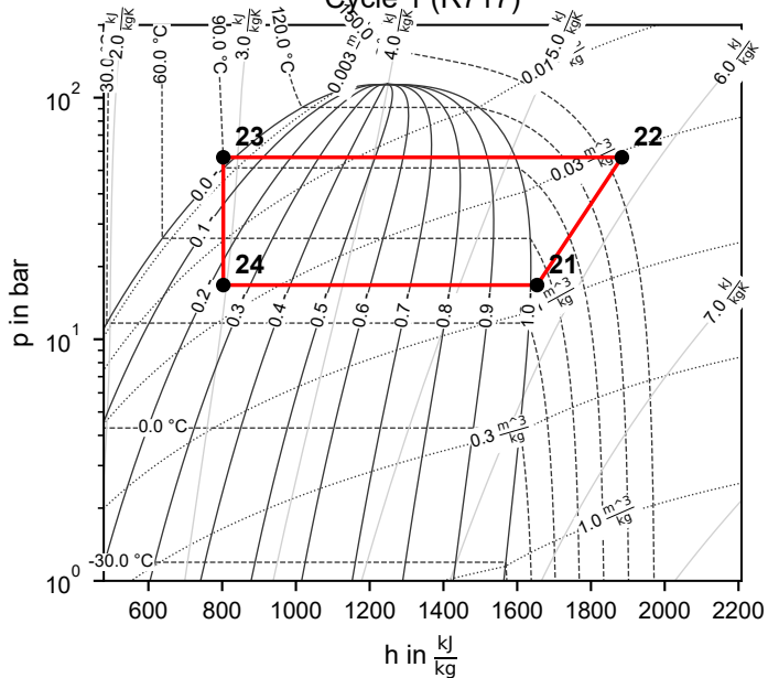
Cycle 1 (R717)
