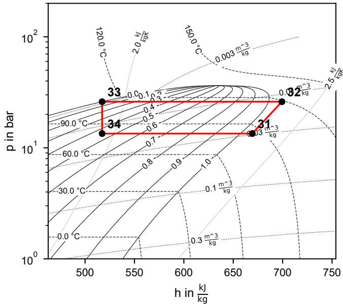
Cycle 2 (R600a)
