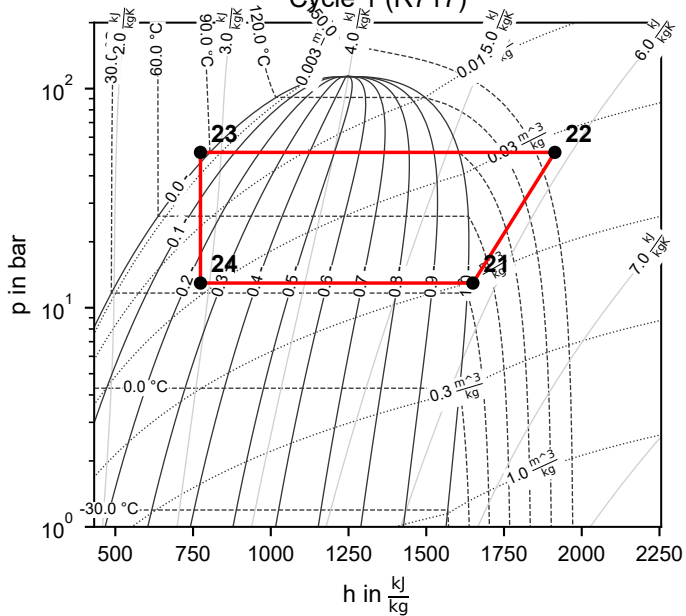
Cycle 1 (R717)
