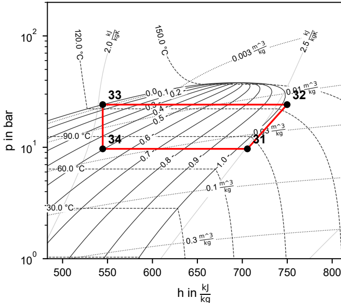
Cycle 2 (R600)
