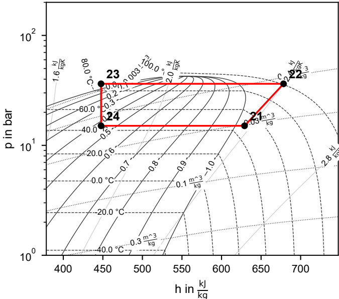
Cycle 1 (R290)
