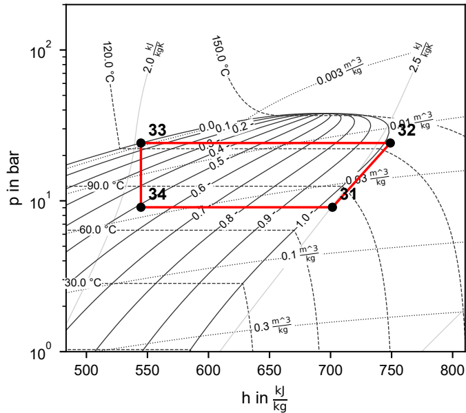
Cycle 2 (R600)
