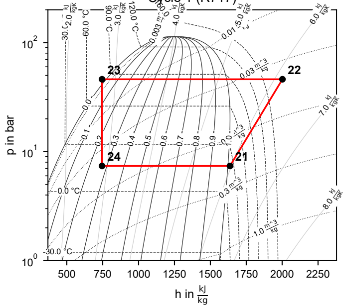
Cycle 1 (R717)
