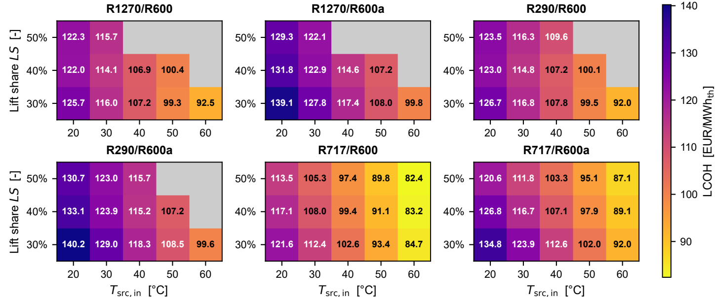
LCOH heatmap per design (heat basis) ( T_{\text{steam}} = 120\text{ }^{\circ}\text{C} )
