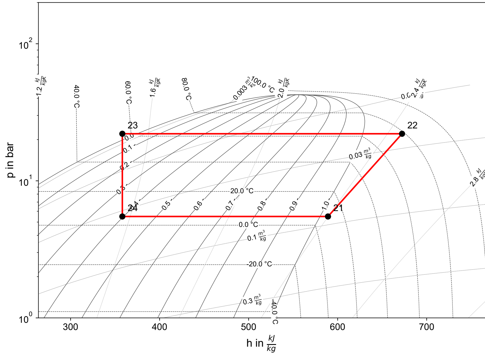
Cycle 1 (R290)
