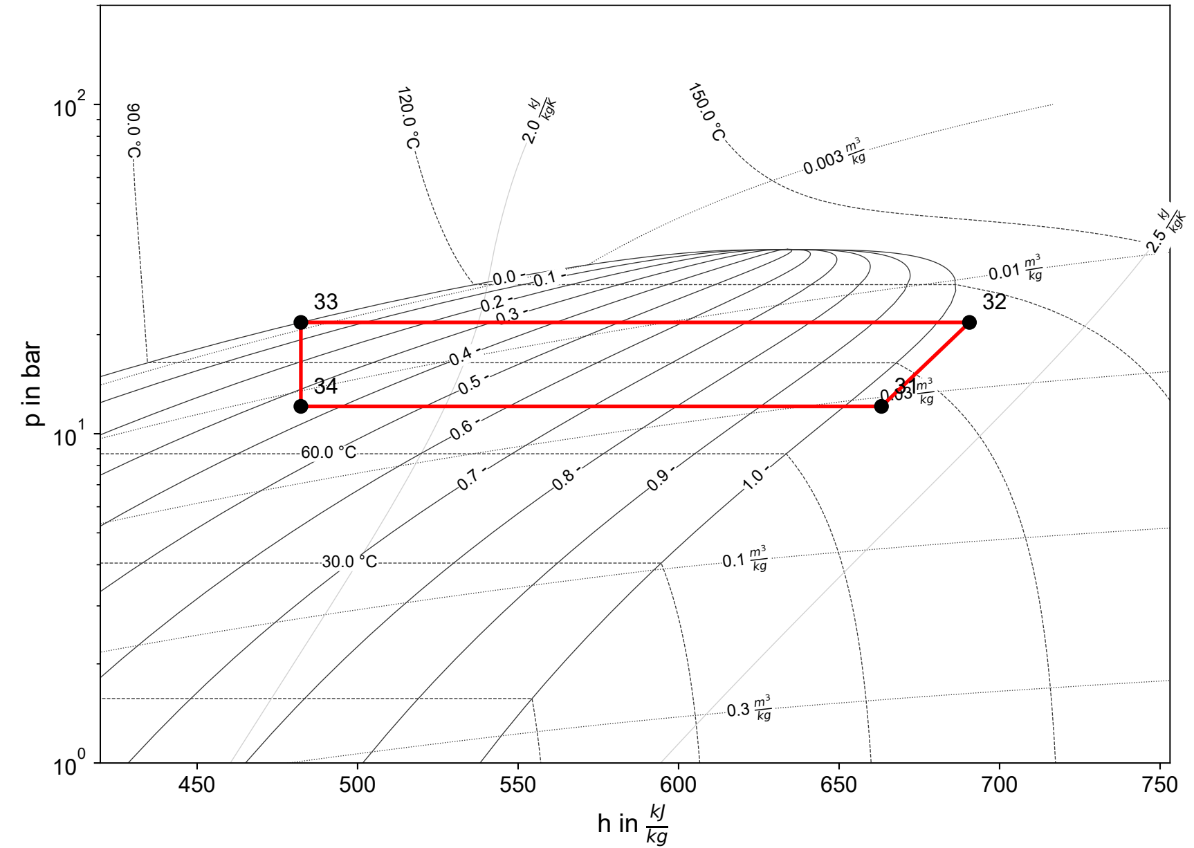
Cycle 2 (R600a)
