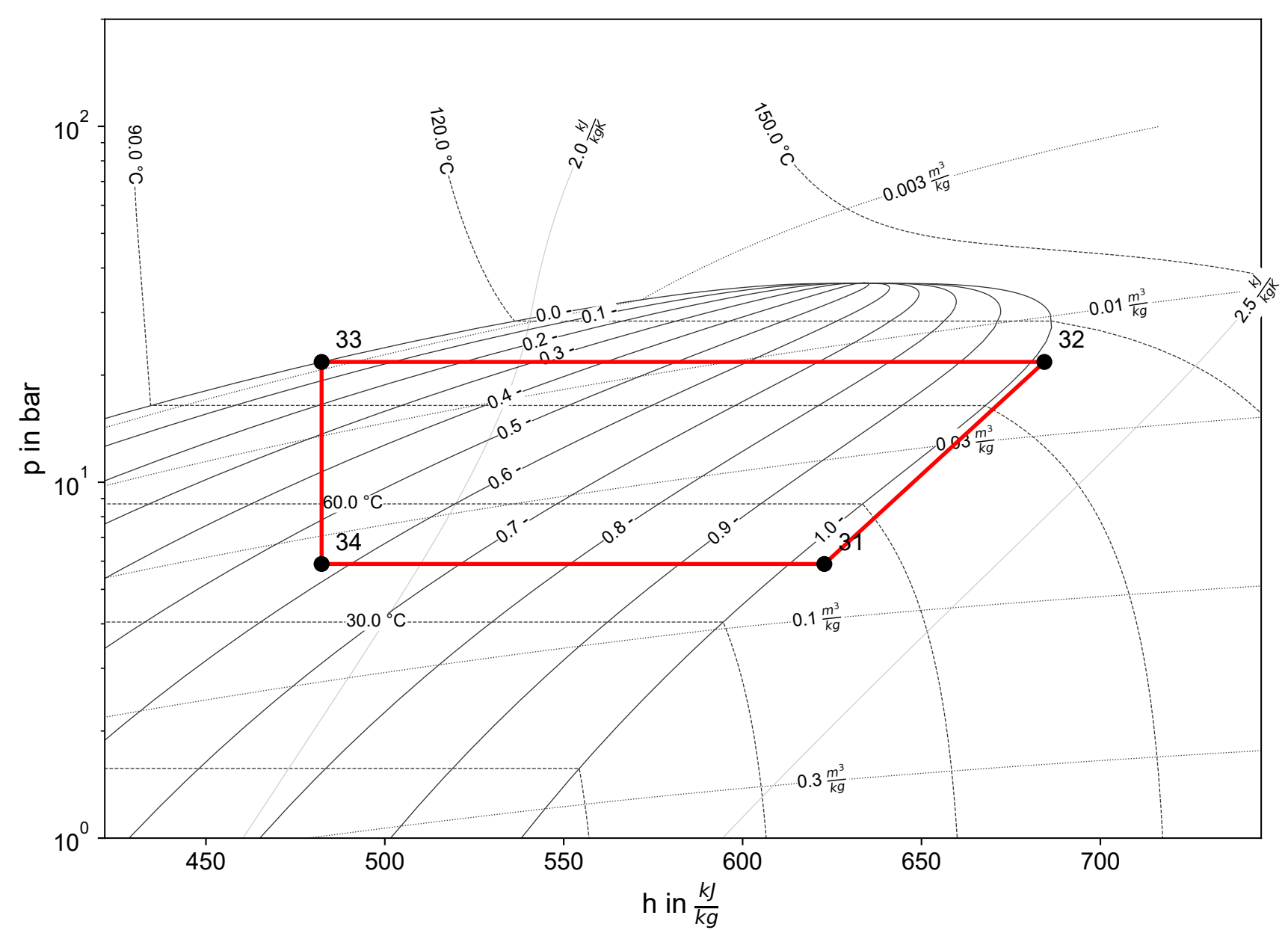
Cycle 2 (R600a)
