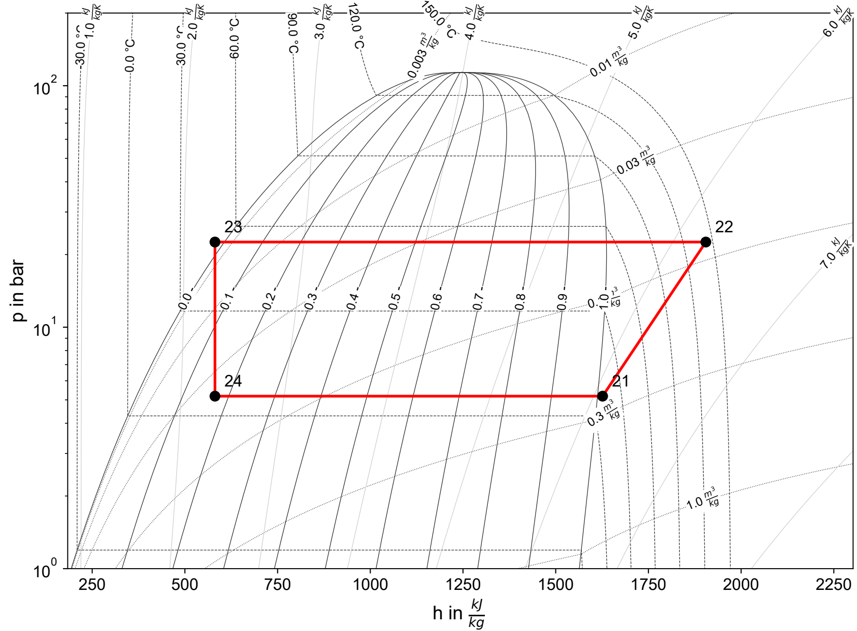
Cycle 1 (R717)
