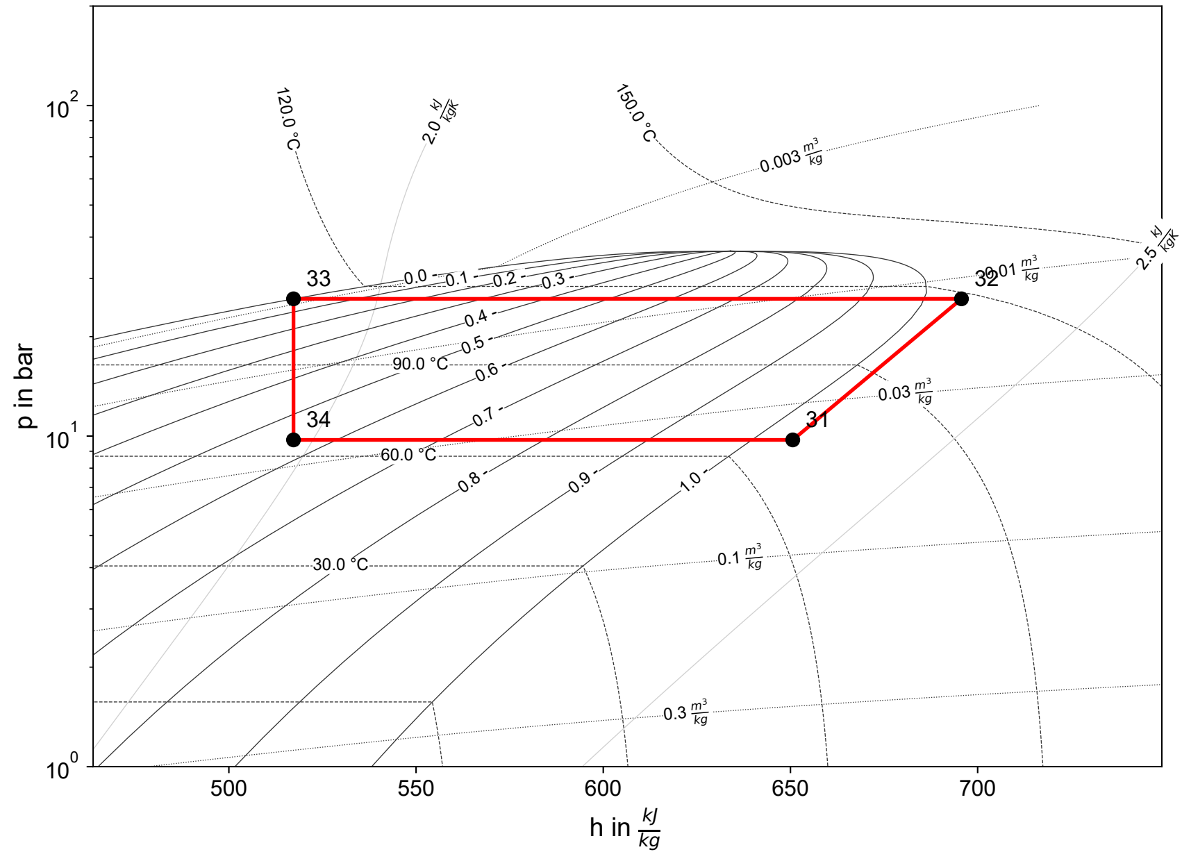
Cycle 2 (R600a)
