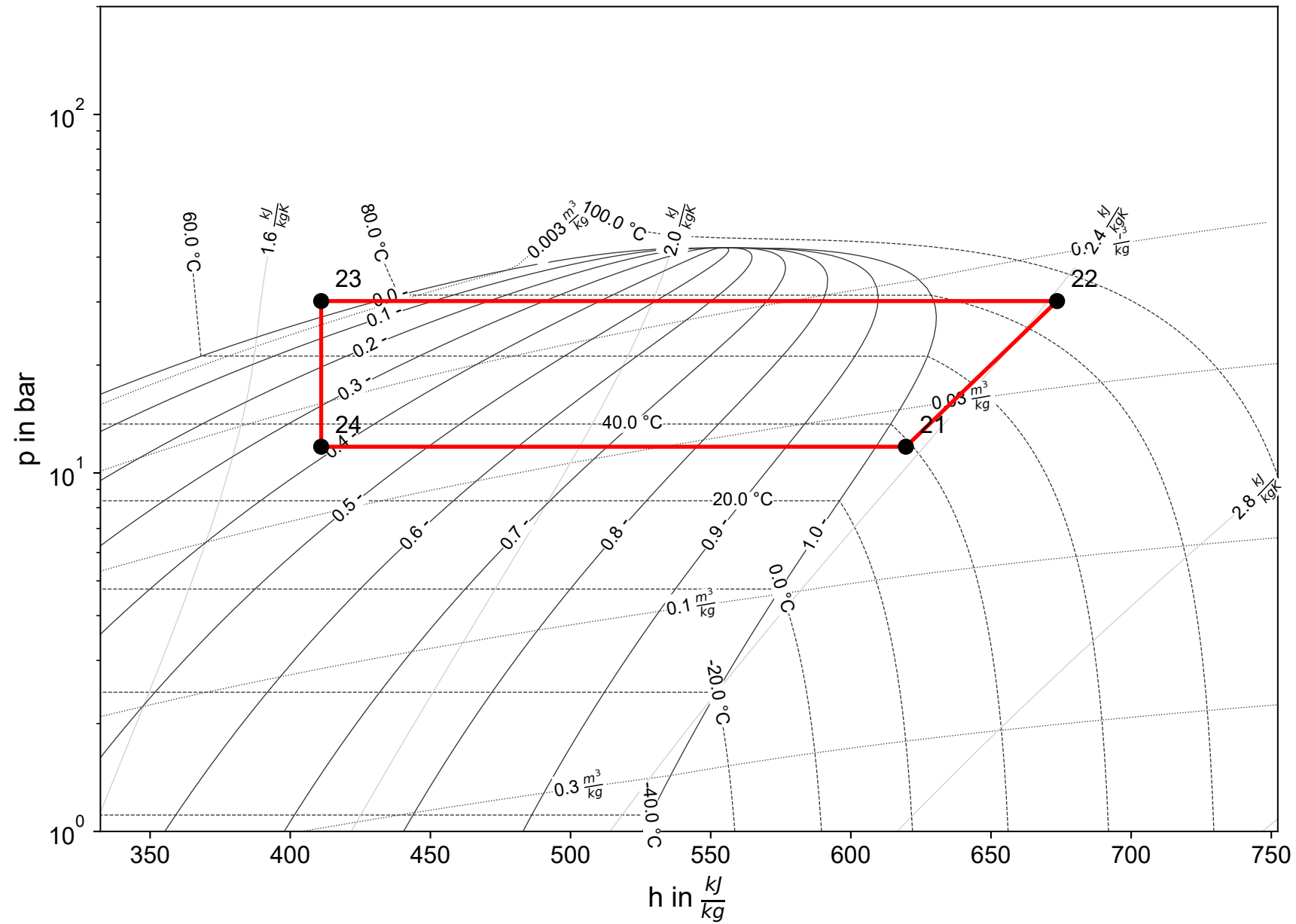
Cycle 1 (R290)
