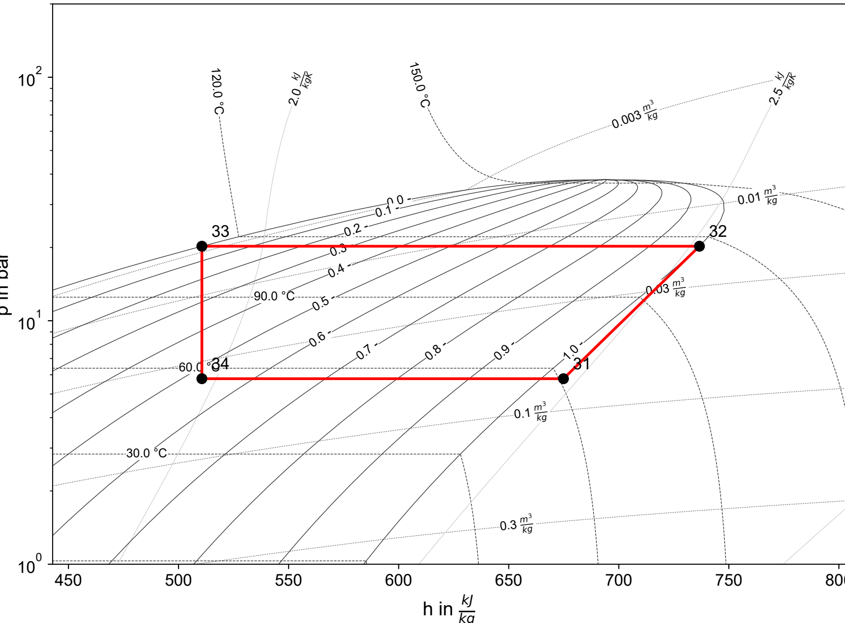
Cycle 2 (R600)
