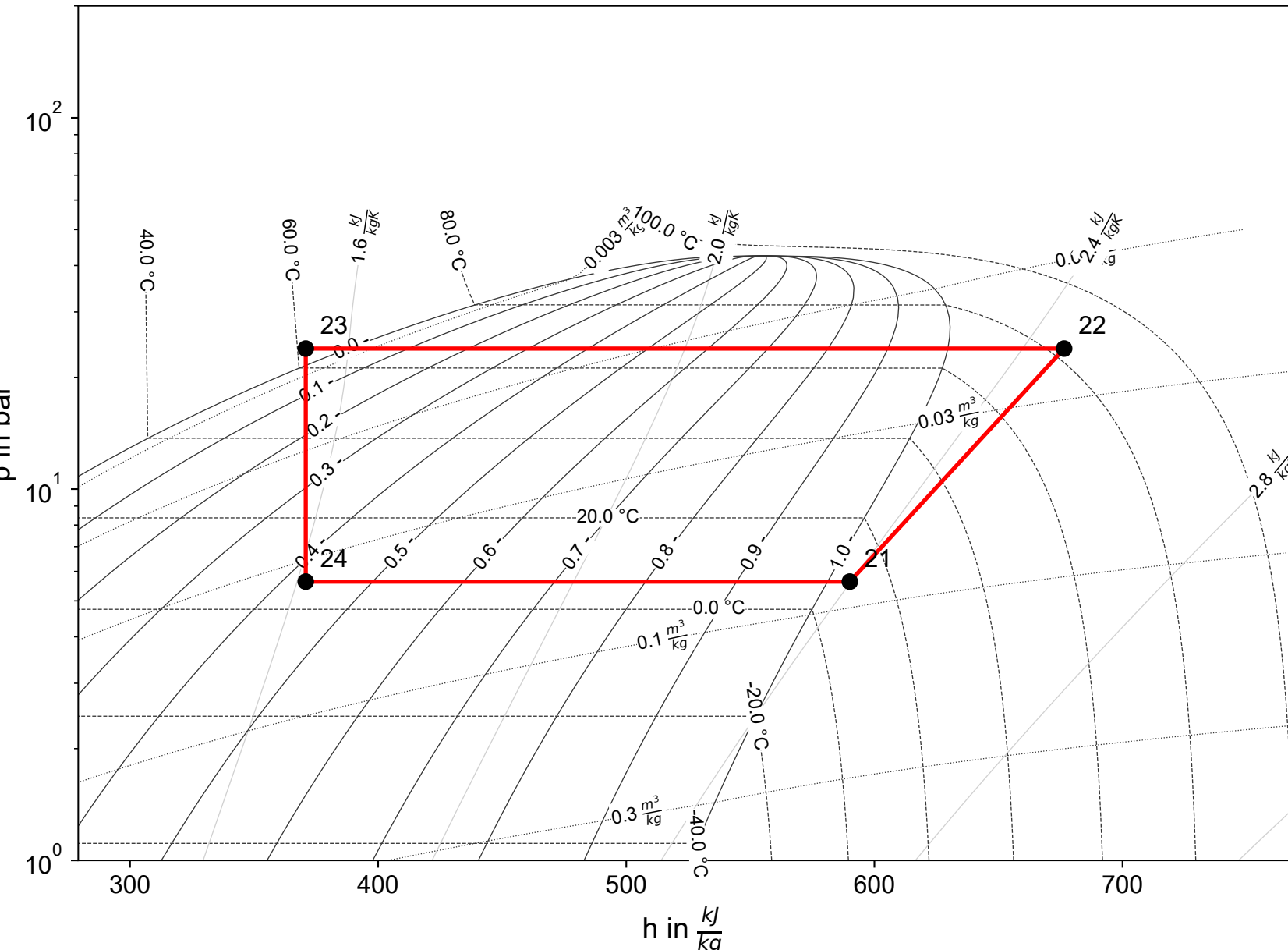
Cycle 1 (R290)
