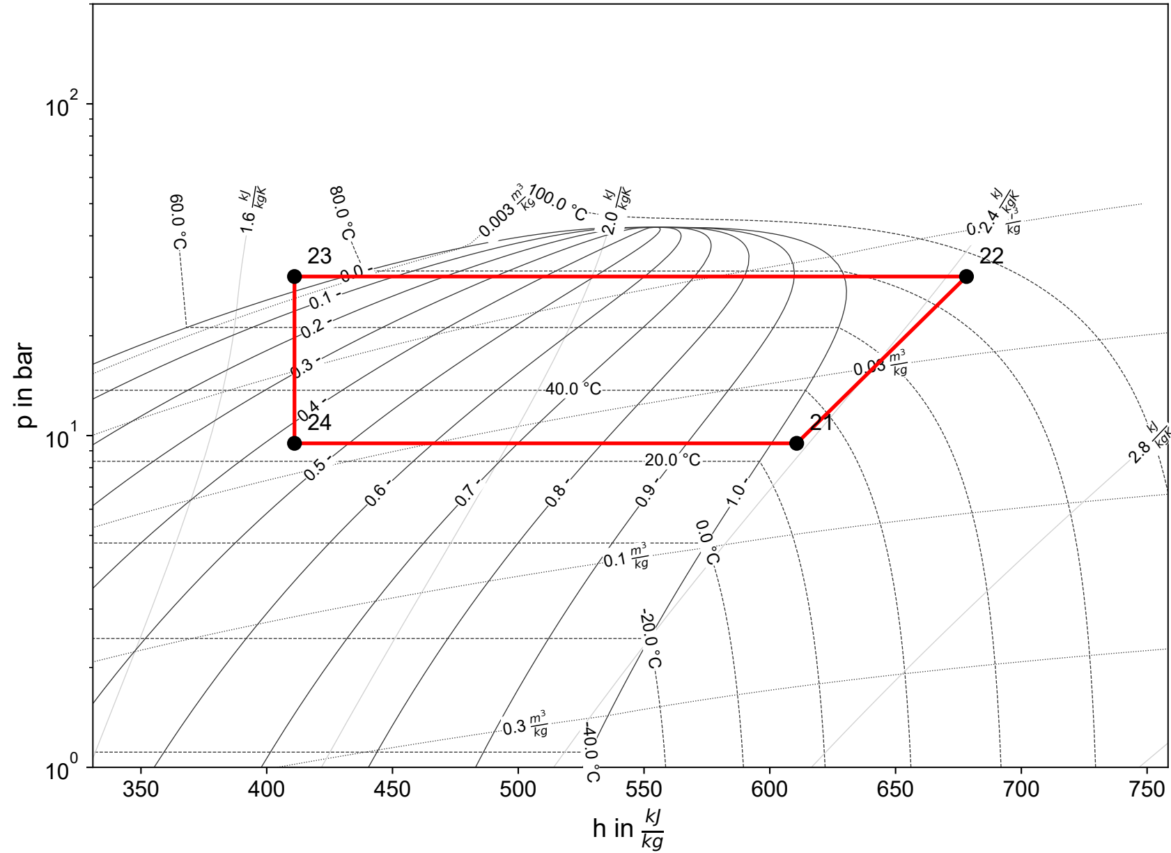
Cycle 1 (R290)
