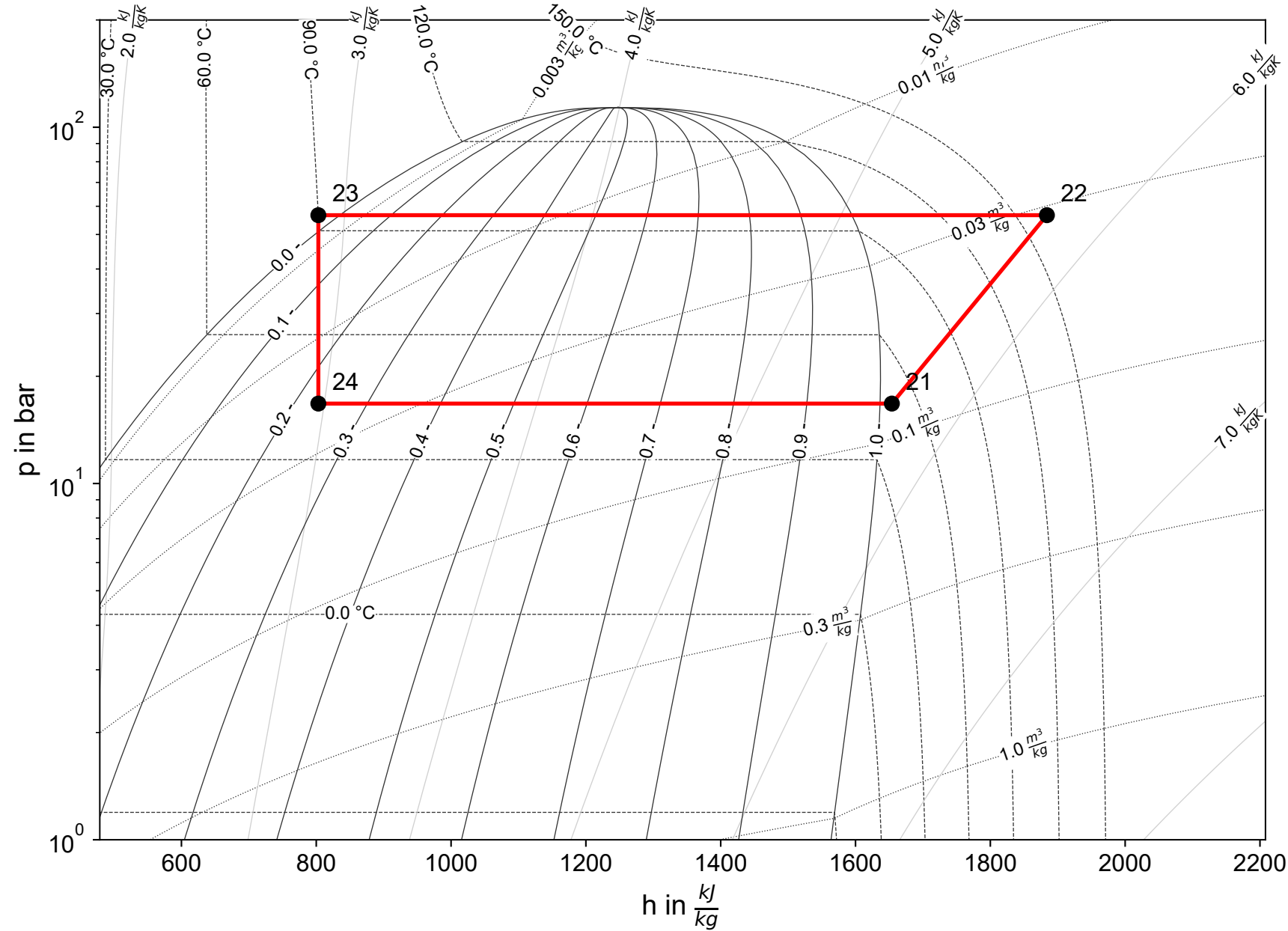
Cycle 1 (R717)
