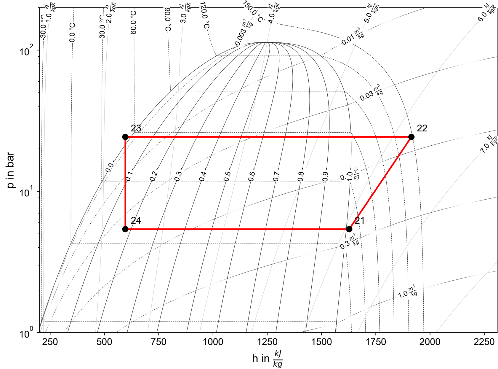
Cycle 1 (R717)
