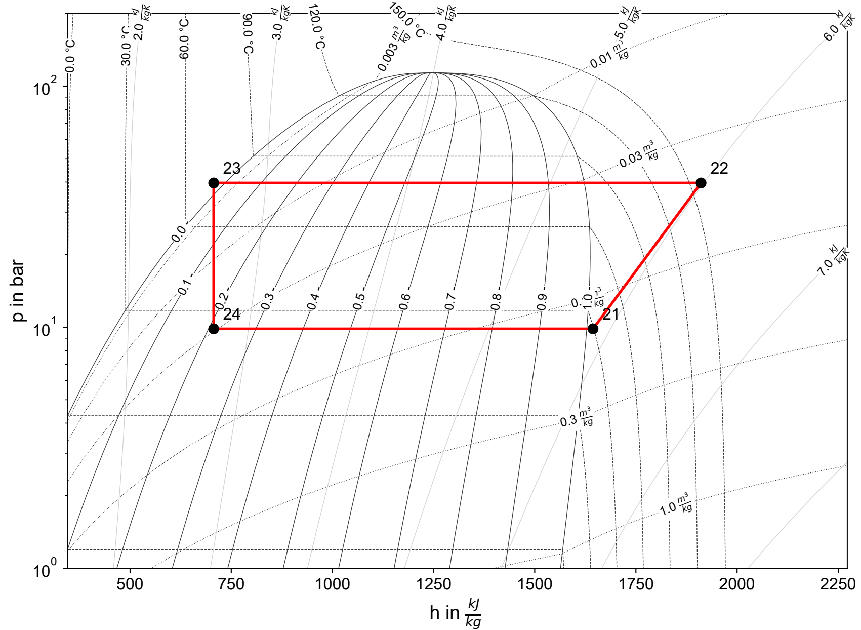
Cycle 1 (R717)
