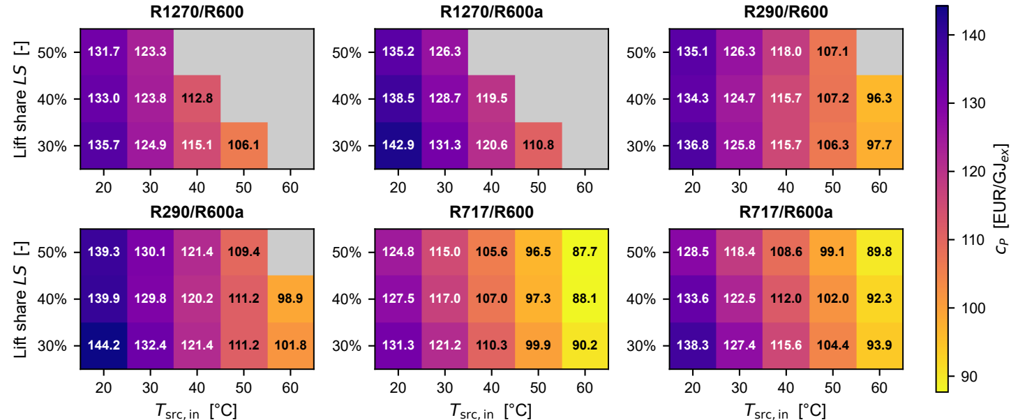
C_p heatmap per design ( T_{\text{steam}} = 110\text{ °C} )
