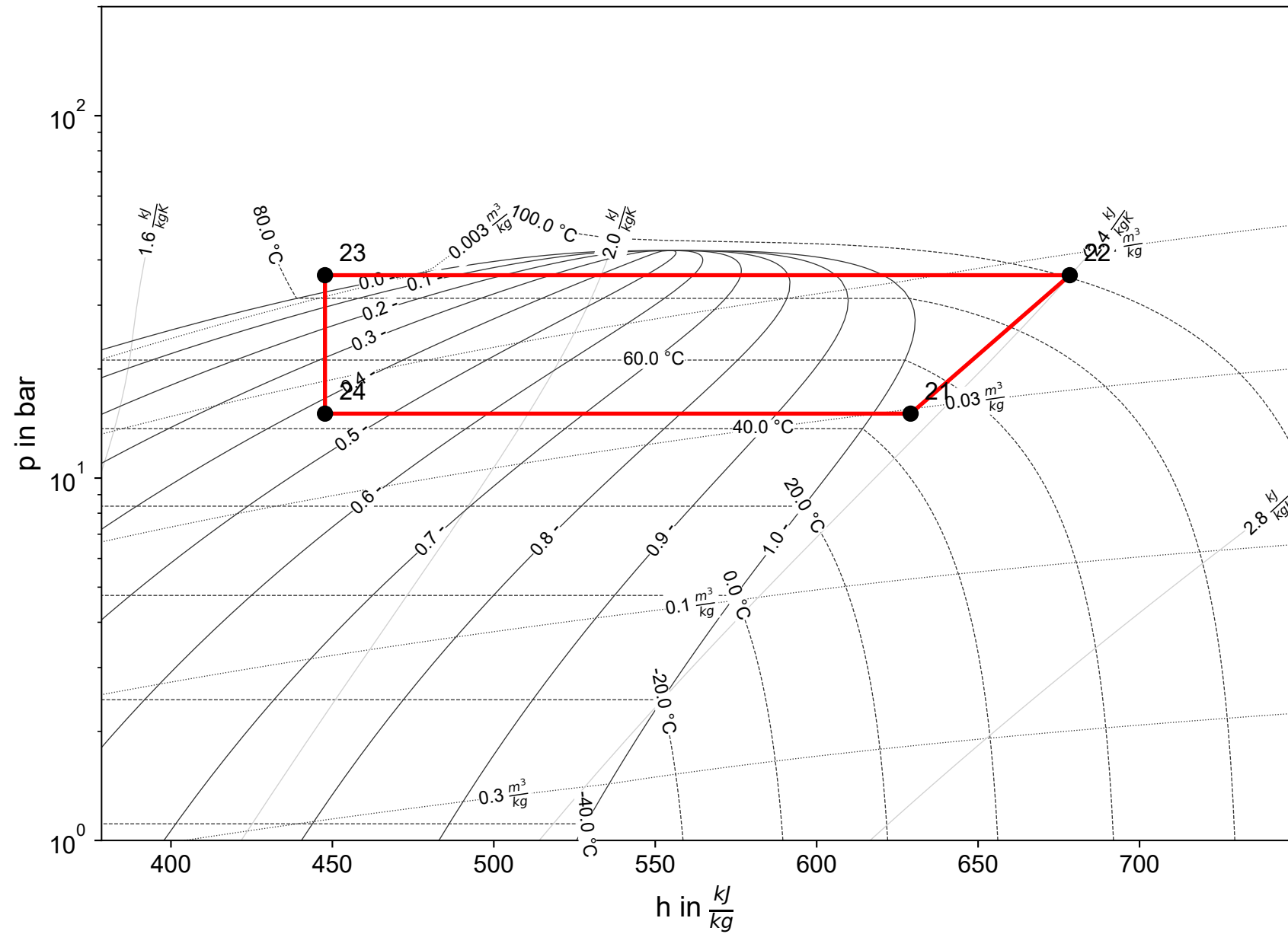
Cycle 1 (R290)
