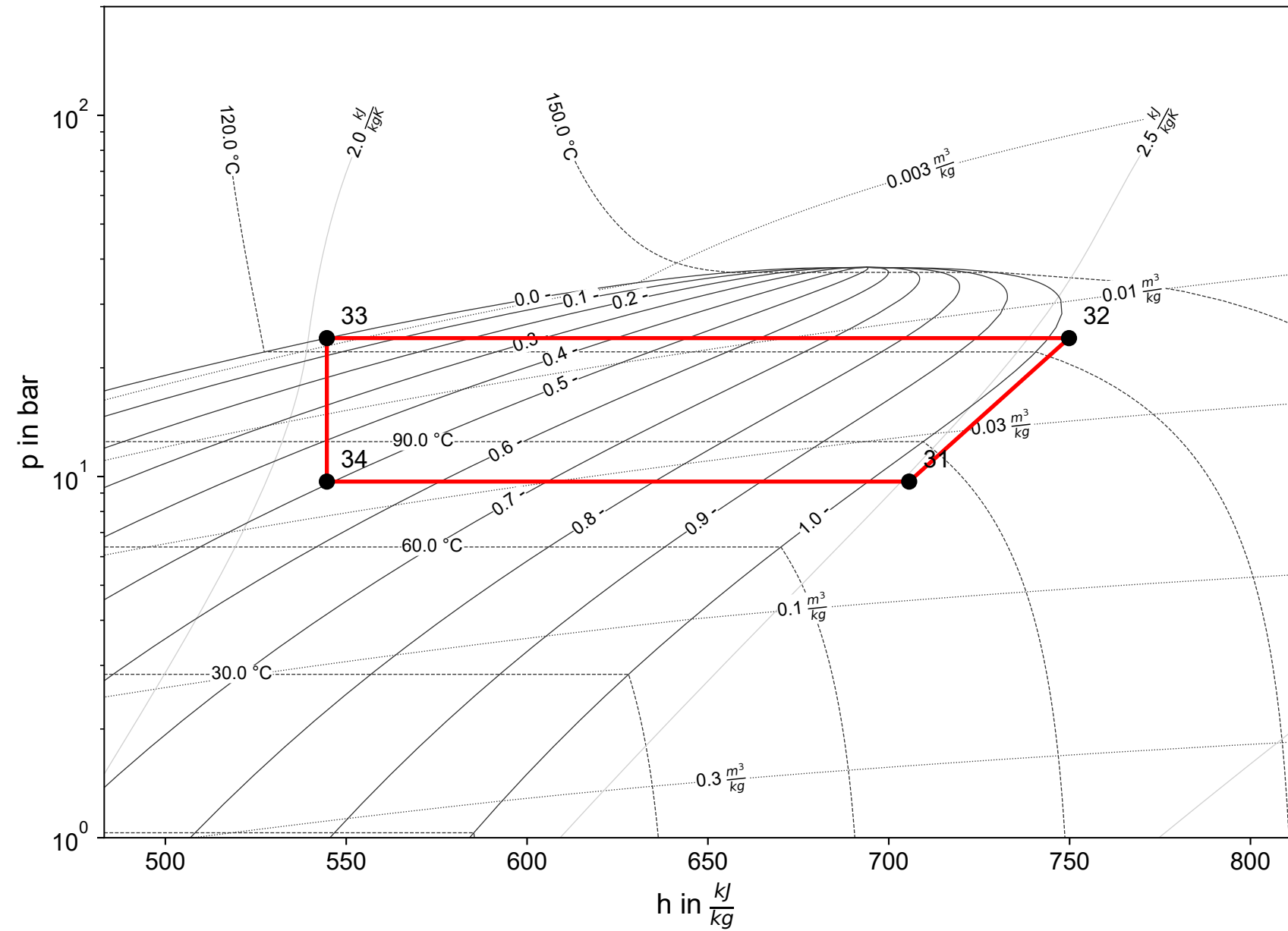
Cycle 2 (R600)
