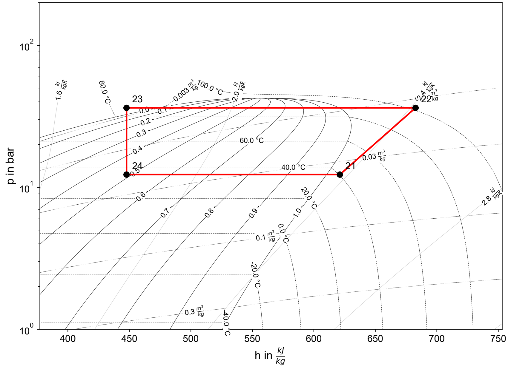
Cycle 1 (R290)
