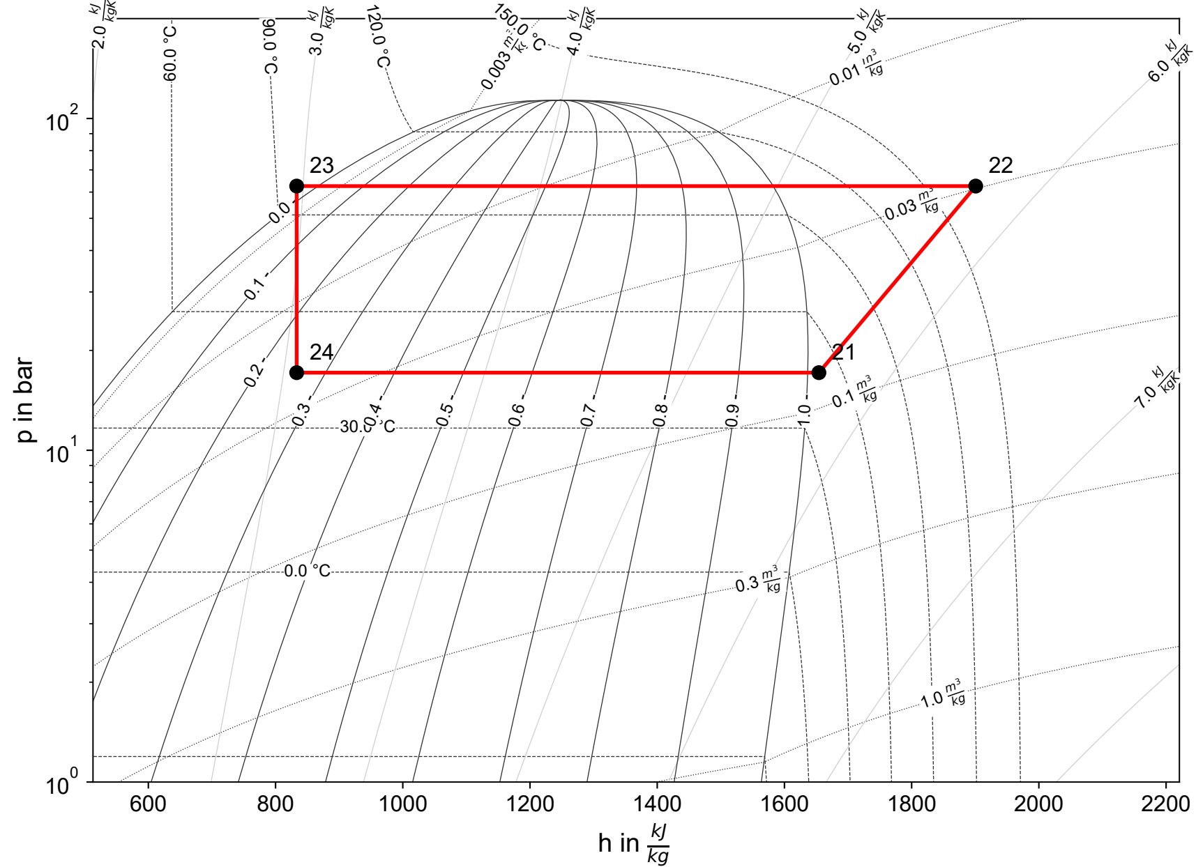
Cycle 1 (R717)
