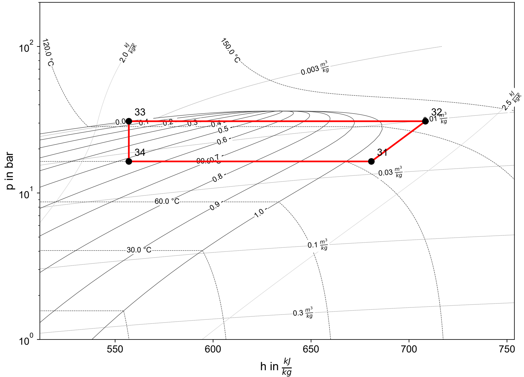
Cycle 2 (R600a)
