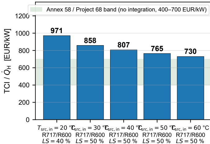
Total capital investment per kW heat
