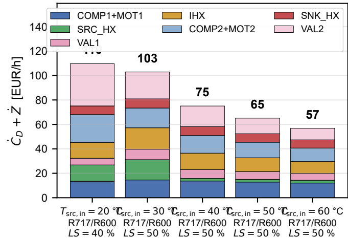
Component cost-rate breakdown
