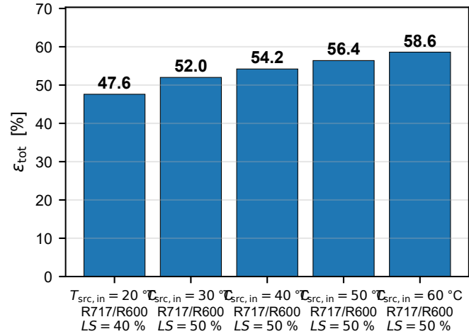
Exergetic efficiency
