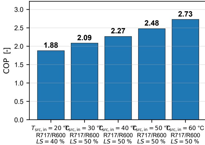
Coefficient of performance
