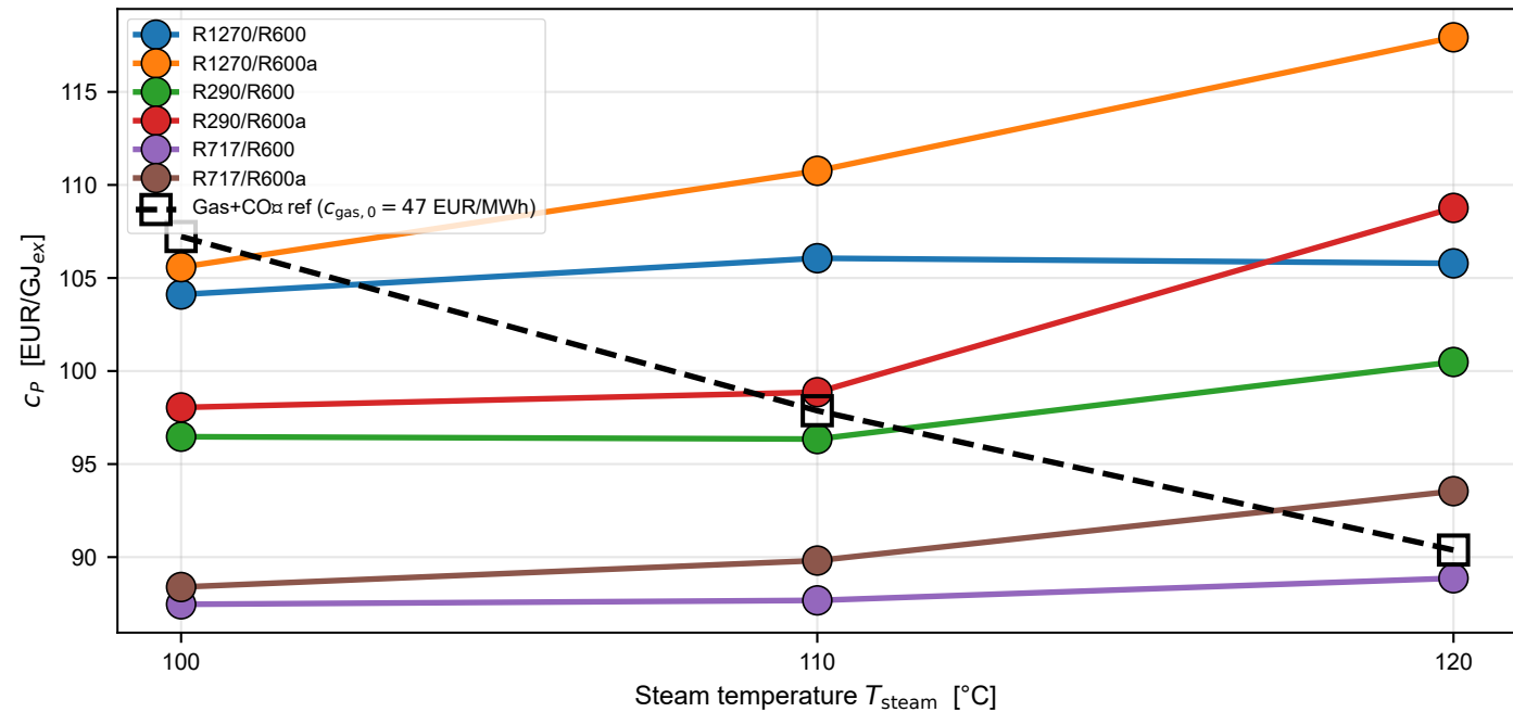
Best c_p per fluid pair vs T_{\text{steam}}
