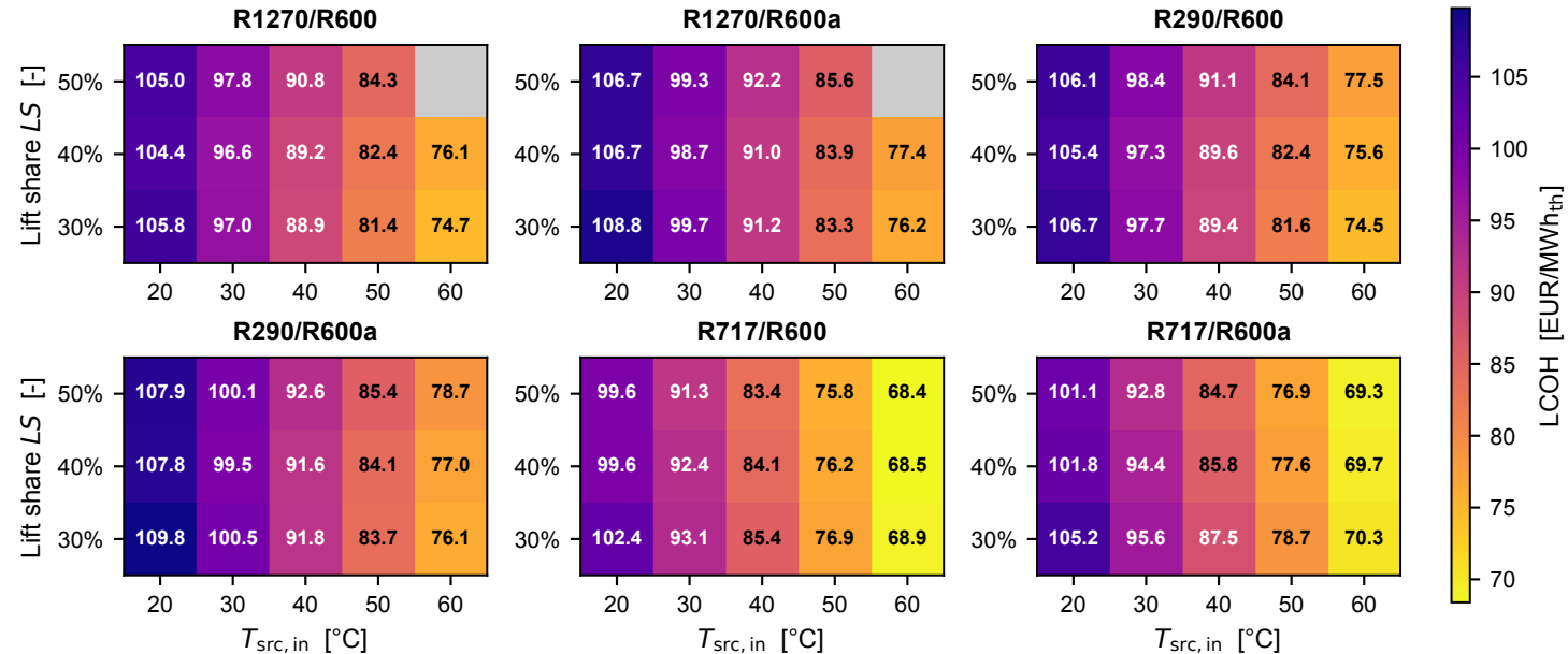
LCOH heatmap per design (heat basis) ( T_{\text{steam}} = 100\text{ }^{\circ}\text{C} )
