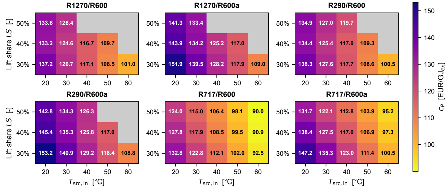
C_P heatmap per design ( T_{\text{steam}} = 120\text{ }^{\circ}\text{C} )
