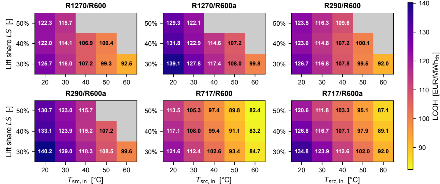
LCOH heatmap per design (heat basis) ( T_{\text{steam}} = 120\text{ }^{\circ}\text{C} )
