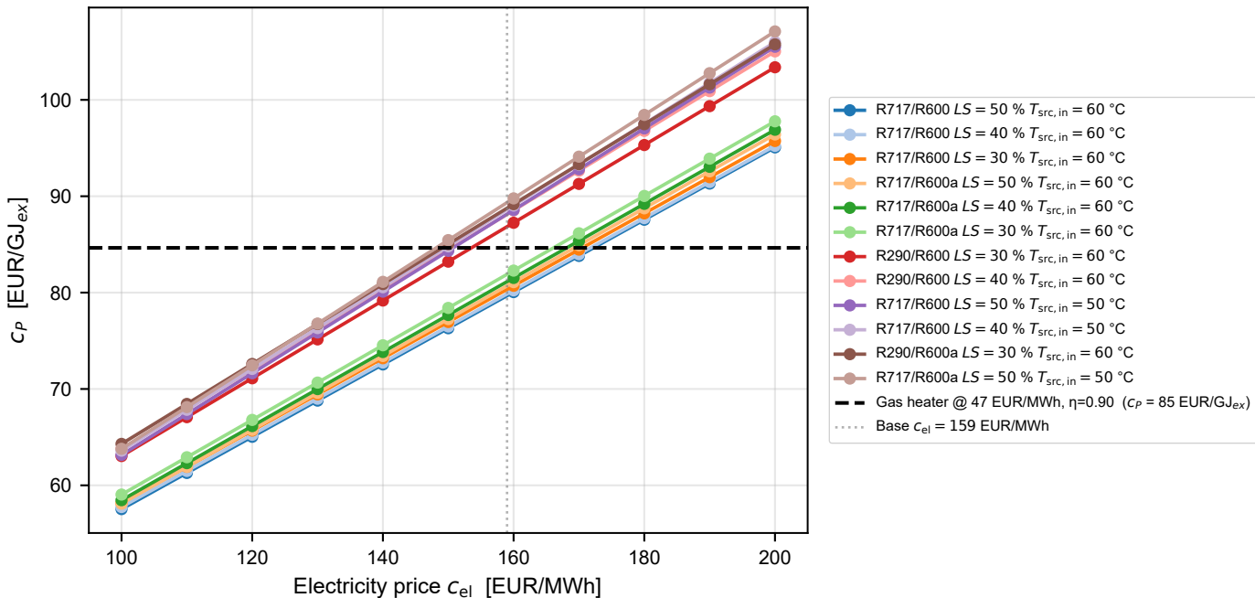
C_P vs electricity price — 12 cheapest designs ( T_{\text{steam}} = 100\text{ }^{\circ}\text{C} )
