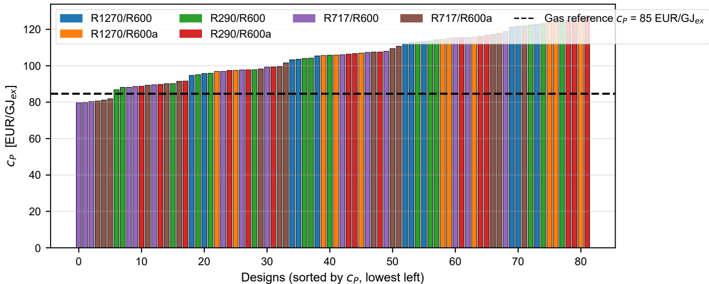
c_p — all OK designs sorted ( T_{\text{steam}} = 100\text{ °C} )
