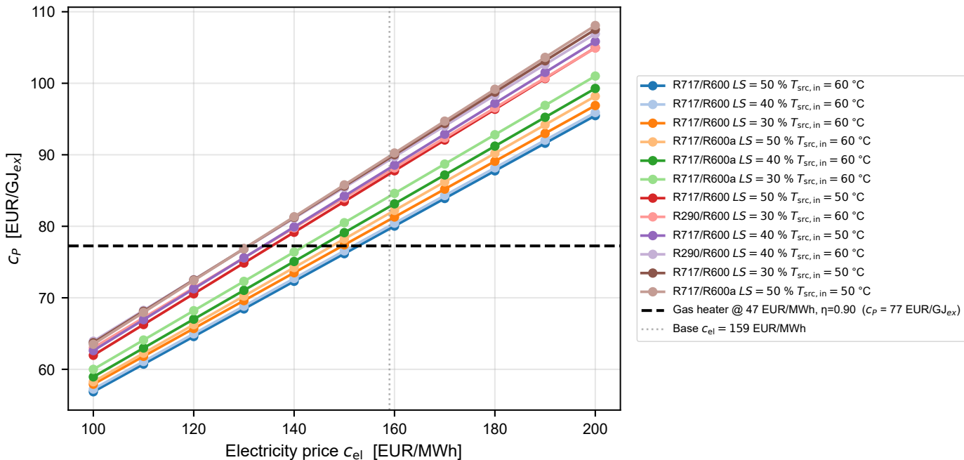
C_P vs electricity price — 12 cheapest designs ( T_{\text{steam}} = 110\text{ }^{\circ}\text{C} )
