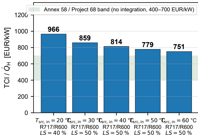
Total capital investment per kW heat
