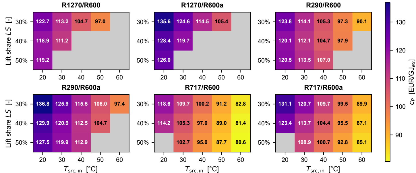
C_p heatmap per design ( T_{\text{steam}} = 120\text{ °C} )
