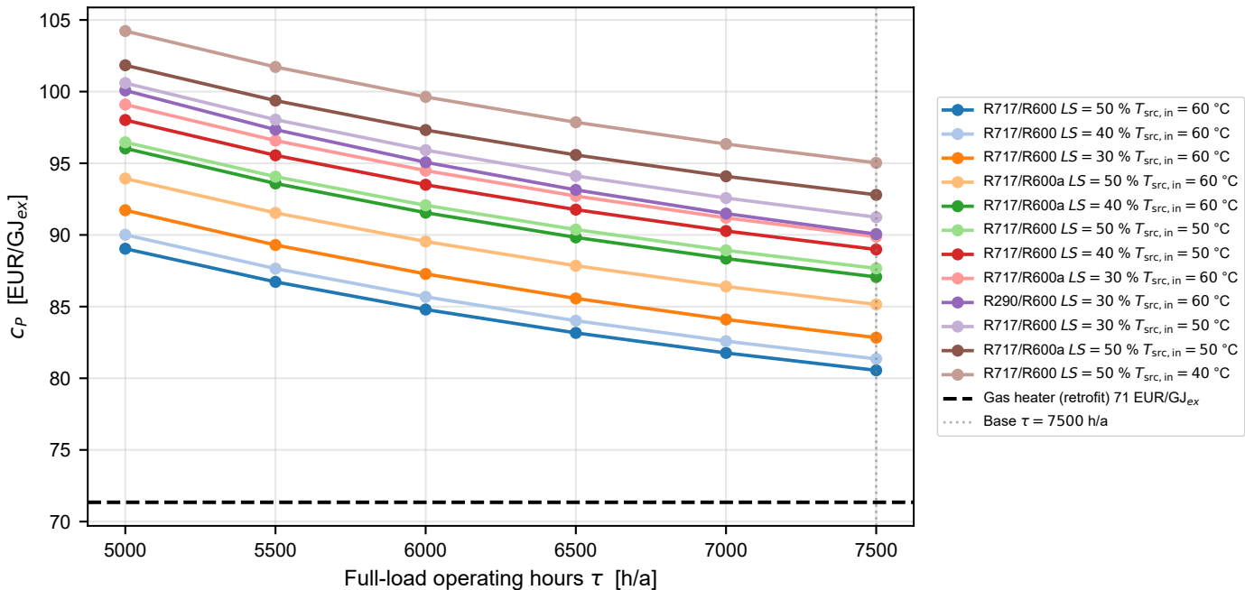
C_P vs full-load hours — 12 cheapest designs ( T_{\text{steam}} = 120\text{ }^{\circ}\text{C} )
